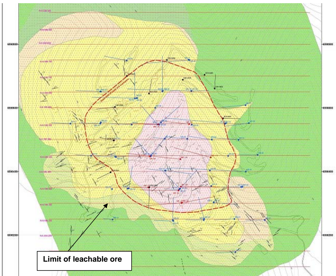
Figure 5: Mollacas copper leach SXEW project : surface geology
